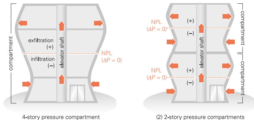
Compartmentalization and winter stack effect
