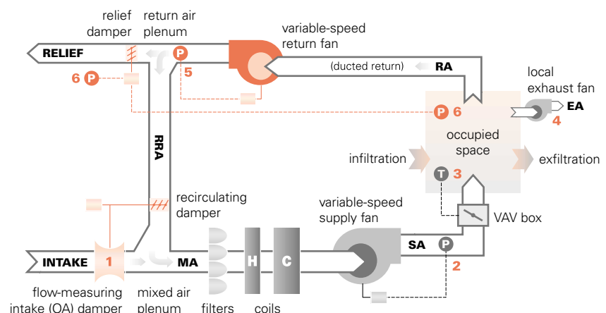
Figure 4. Typical VAV system with central return fan
