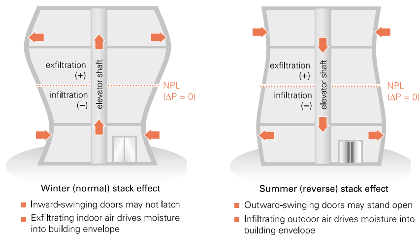
Figure 1. Stack effect and building pressure
